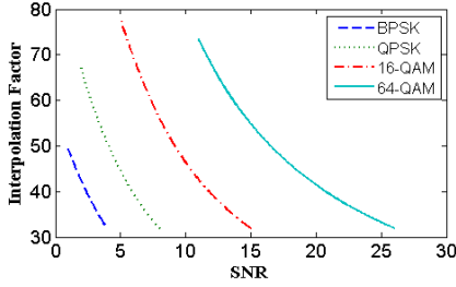
Fig. 5: Mapping rules for interpolation/decimation factor with varied SNR.
