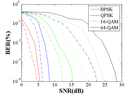
Fig. 11: TiM's BER performance with varied SNR.
