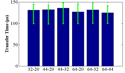
Fig. 7: Time delay of decreasing interpolation.
