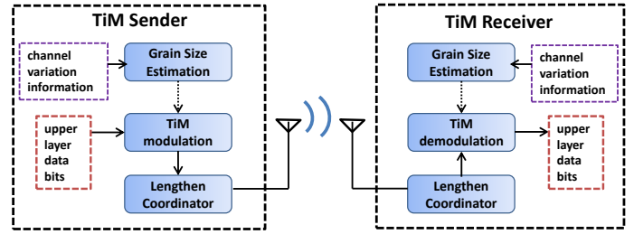
Fig. 8: High-level architecture of TiM’s sender and receiver.
